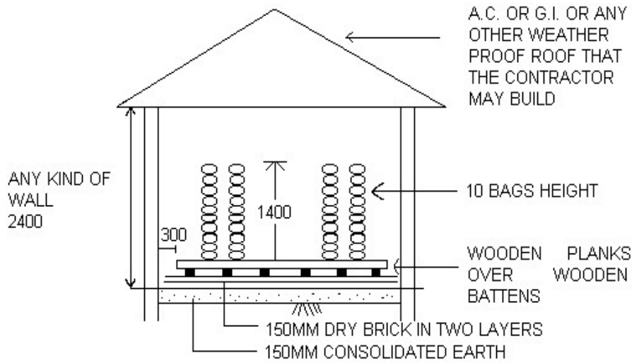
SECTION AB
