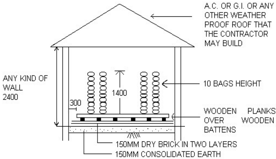
SECTION AB
